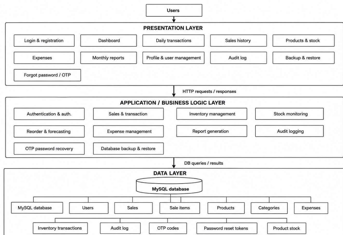
Figure 4.3 Architecture Diagram
